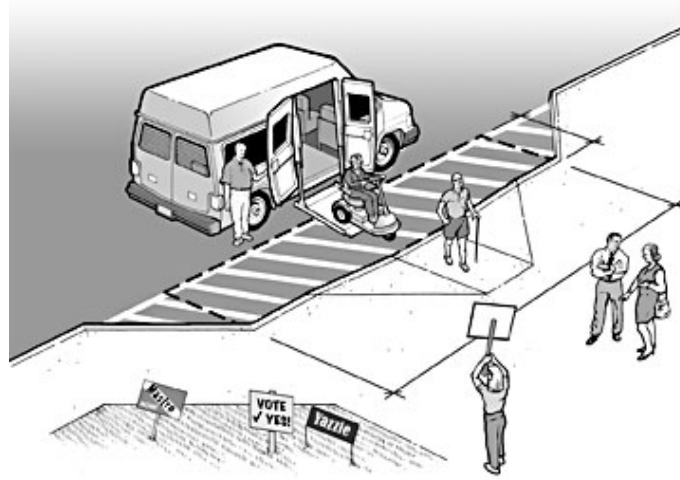
Accessible passenger drop-off and loading area
